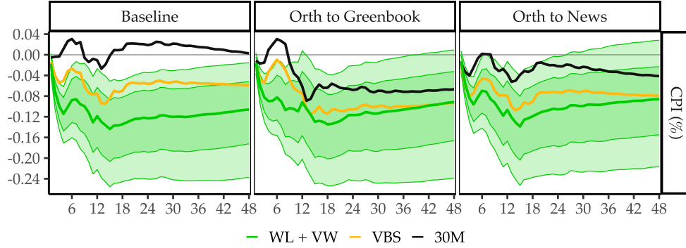
(a) VAR(12)
