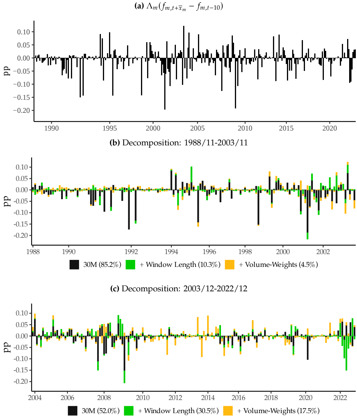
Figure 6: Volume-Based Surprise
